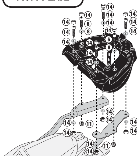
M6M PLATE
