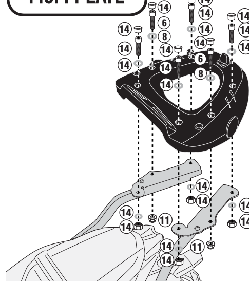
M5M PLATE
