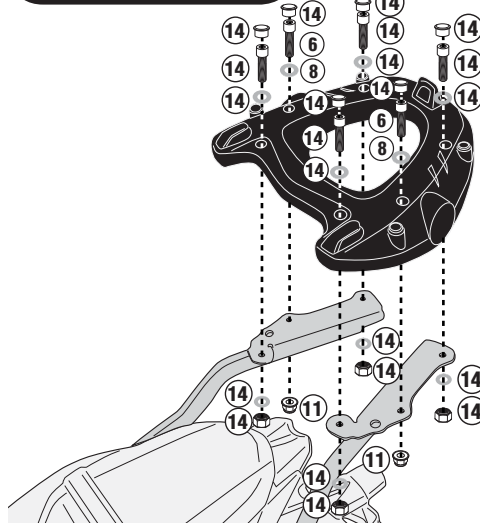
M5M PLATE
